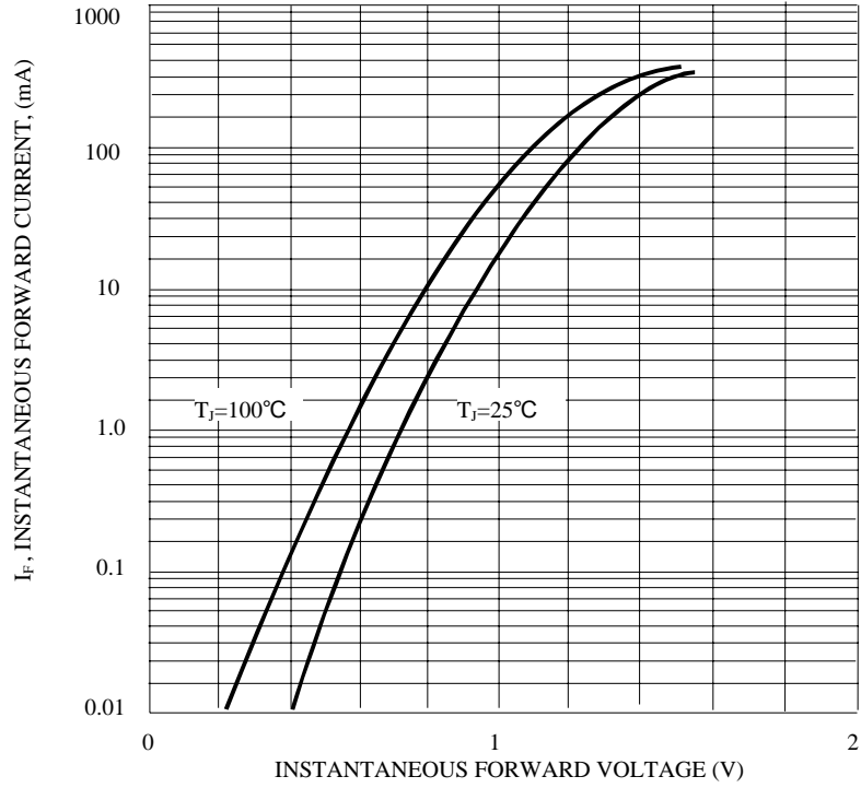
FIG.1 - FORWARD CHARACTERISTICS
