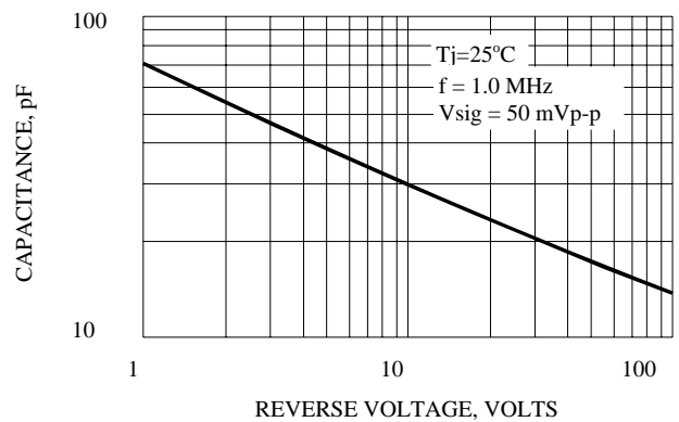
FIG. 5-TYPICAL JUNCTION CAPACITANCE
