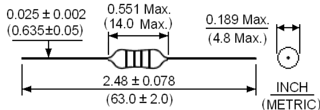
Mechanical drawing
